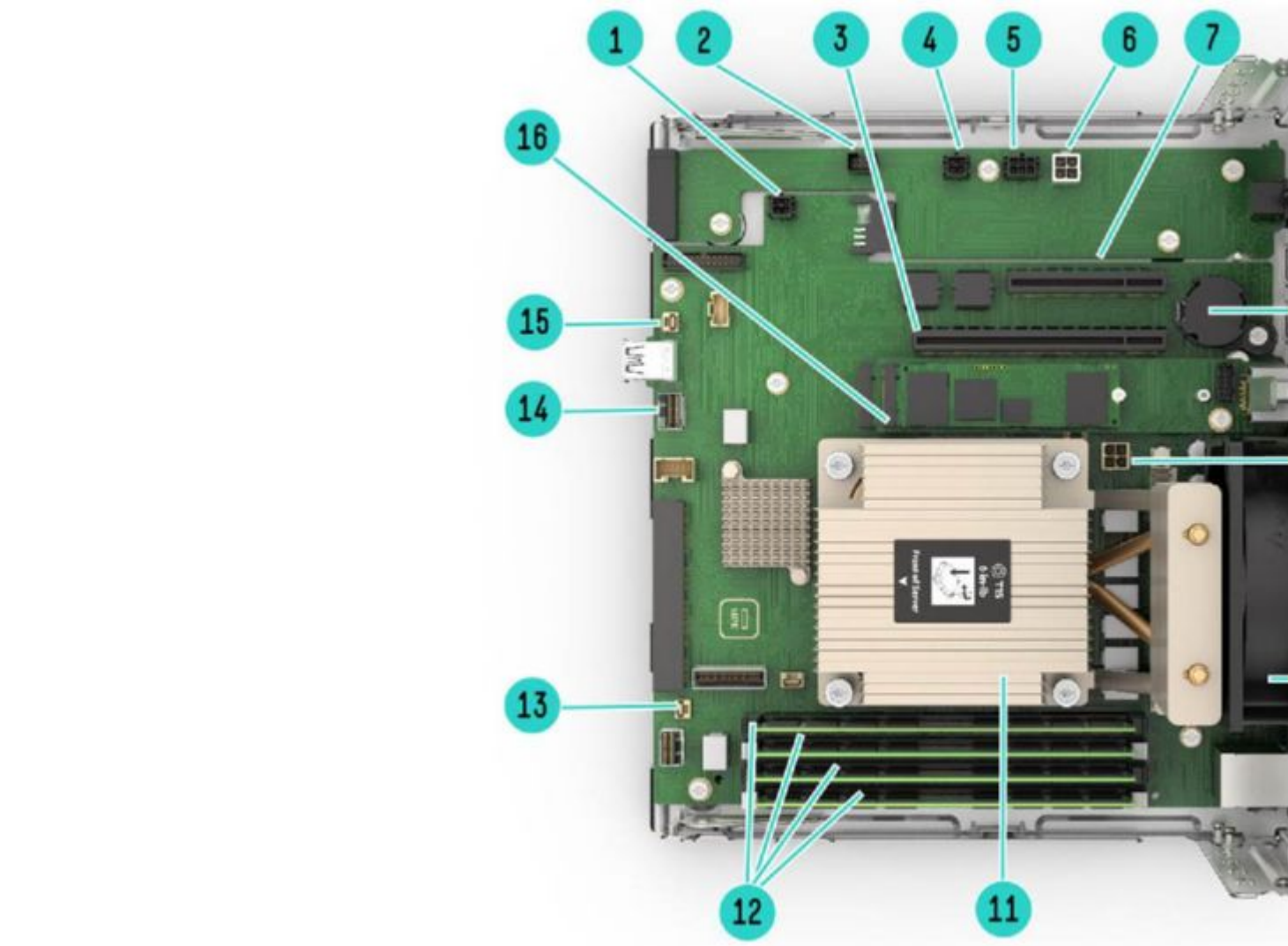
Mainboard View (Internal)
